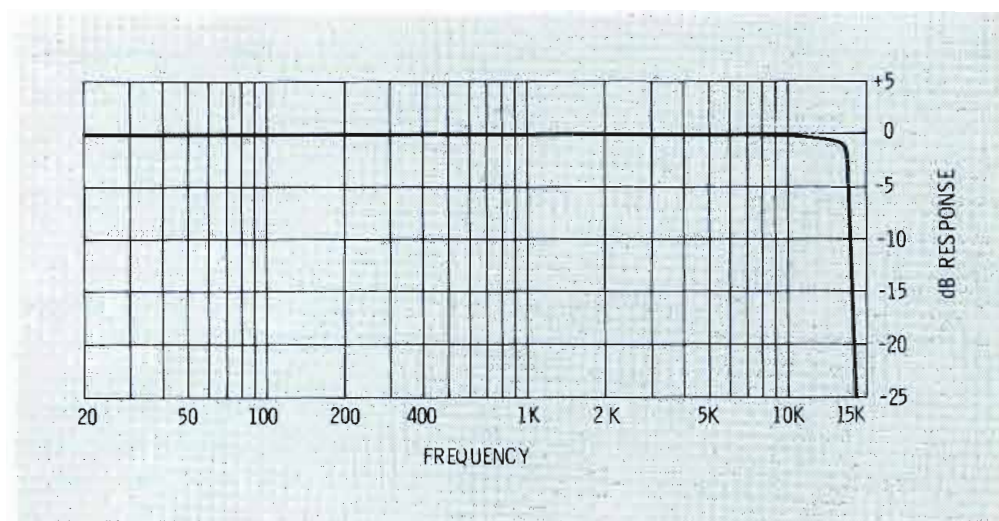
Fig. 2 Bandpass characteristics used for the distortion measurements.
